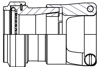
CABLE CLAMP OPTION
