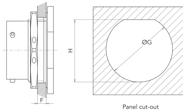
Panel cut-out
