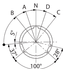
View from front face of receptacle
