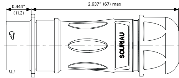
Fig. 2 Cable diameter acceptance from 0.157" to 0.275" (4 to 7)
