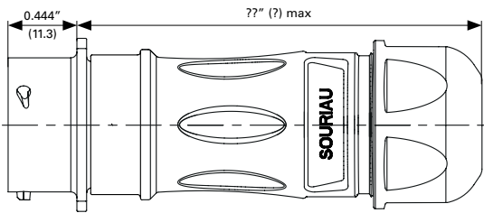
Fig. 2 Cable diameter acceptance from 0.393" to 0.511" (10 to 13)
